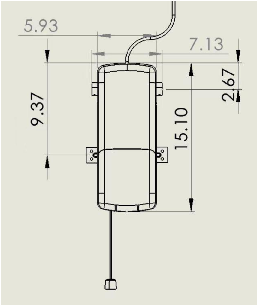
Guardian Model 928: Exterior Dimensions
